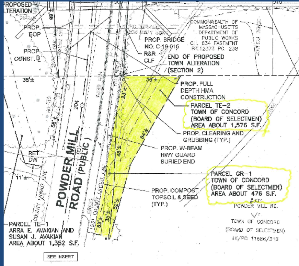
Plan showing location of the easements for the Rail Trail over Town-owned land on Powder Mill Road.
