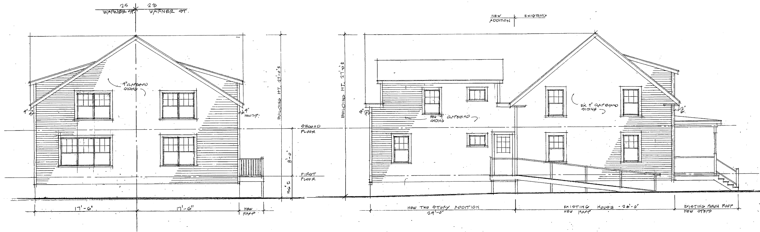
PROPOSED LEFT SIDE ELEVATION - RIGHT SIDE SIMILAR (SIDE VIEW OF 23 WARNER ST.) 1/4" = 1'-0"
