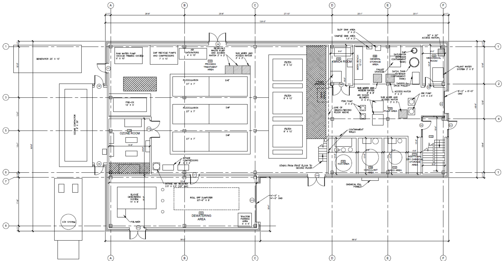
Filtration Facility Floor Plan – Ground Floor
