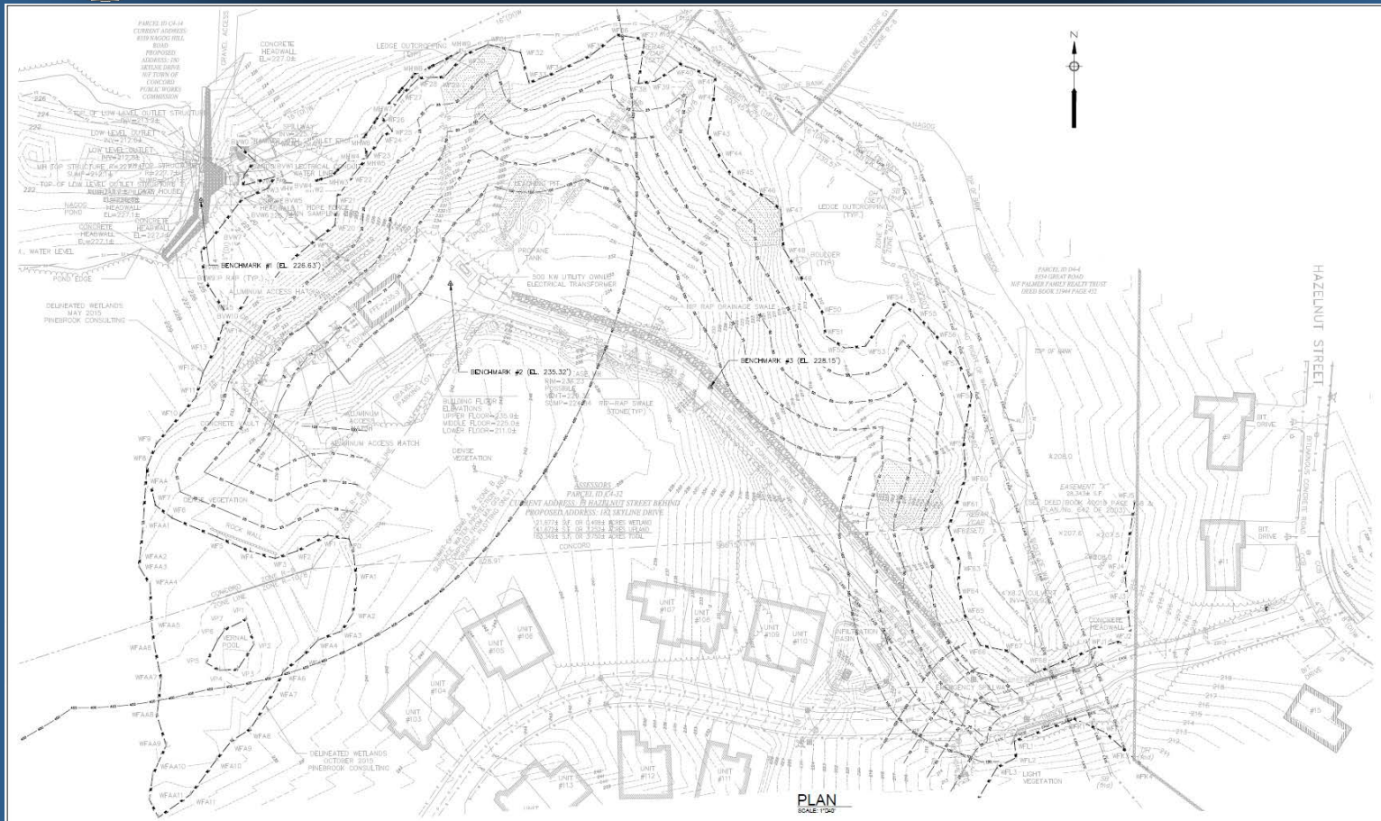
Existing Treatment Plant Site Conditions
