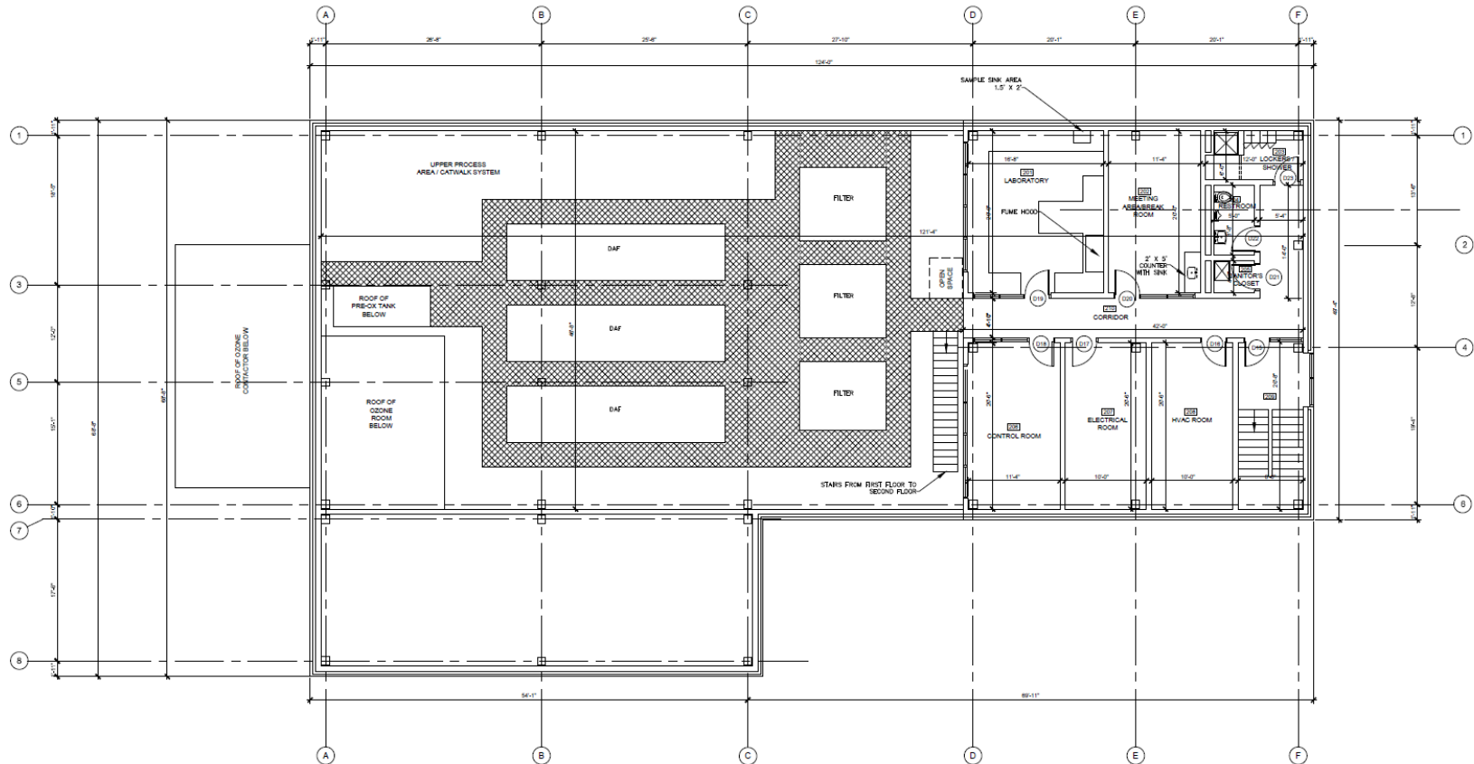
Filtration Facility Floor Plan – Second Floor
